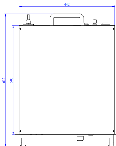
Left View
